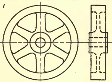
CAST IRON FLY WHEEL.
